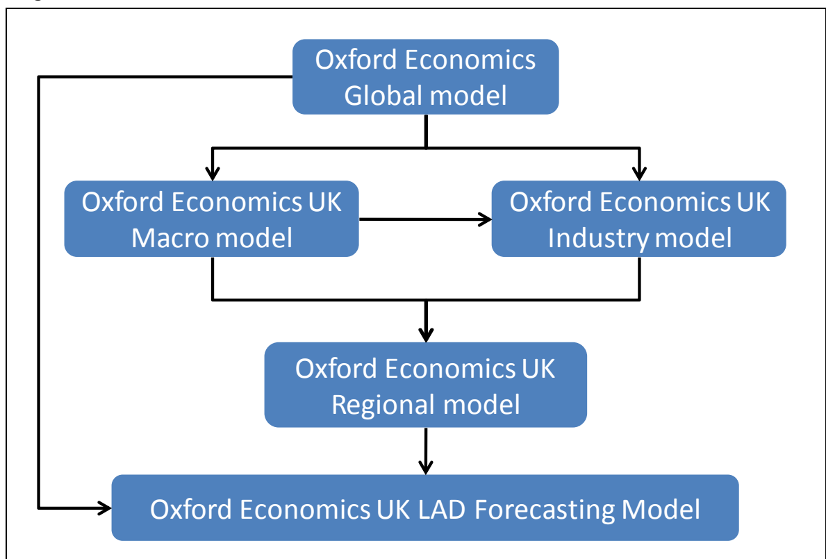
Figure 19: Hierarchical structure of Oxford Economics' suite of models
